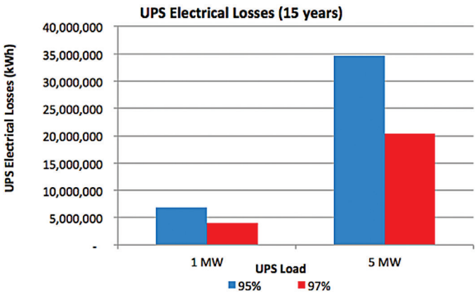
Figure 3. UPS Electrical Losses In kWh
